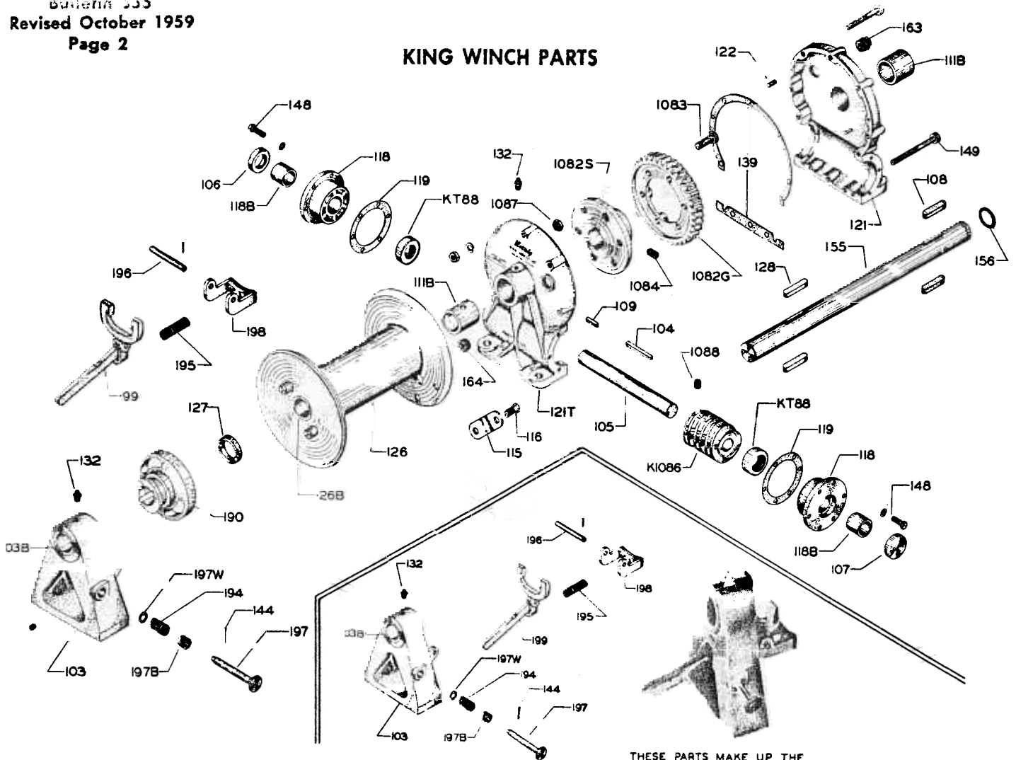
THESE PARTS MAKE UP THE 103A BRACKET ASSEMBLY
